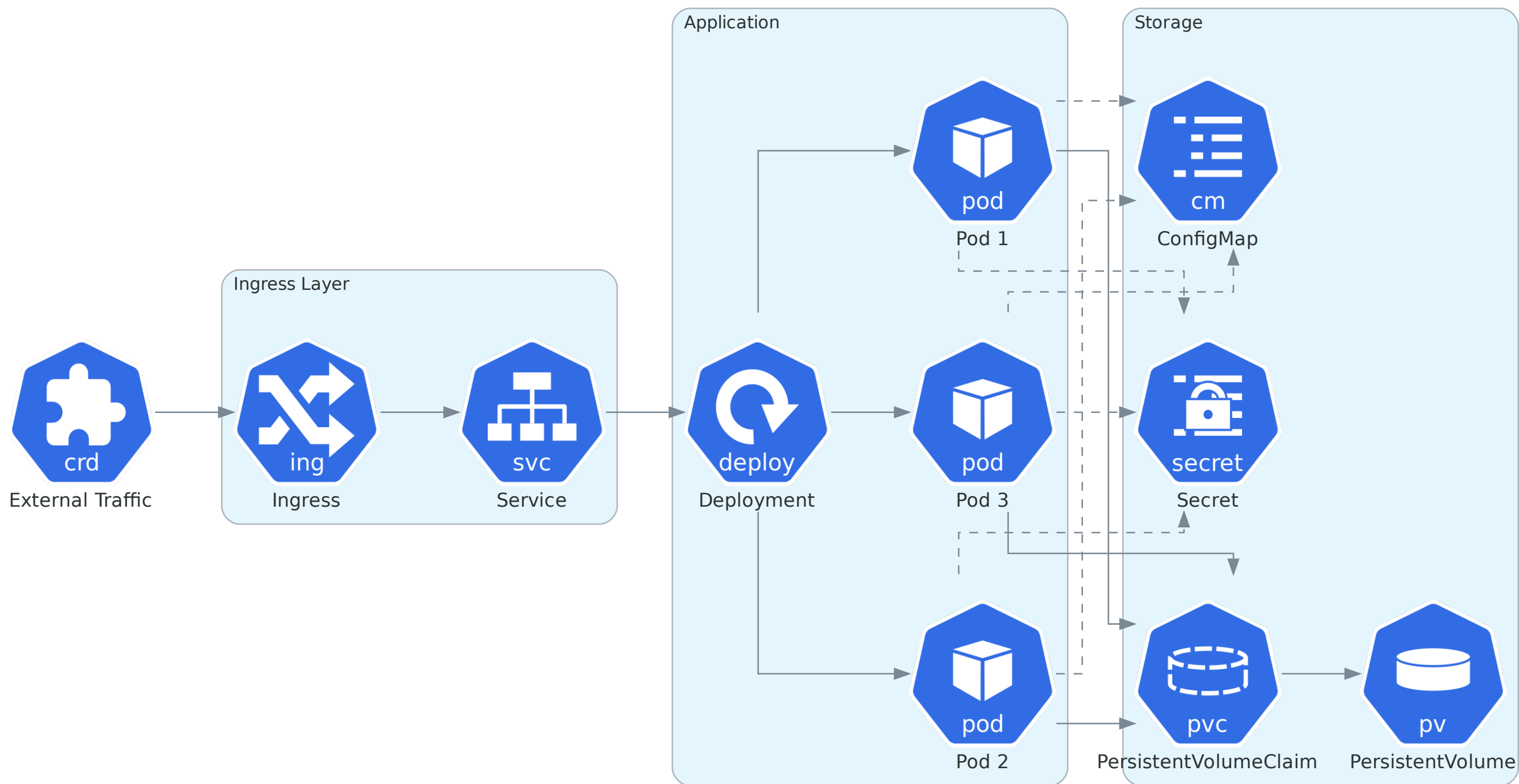
Kubernetes Deployment
